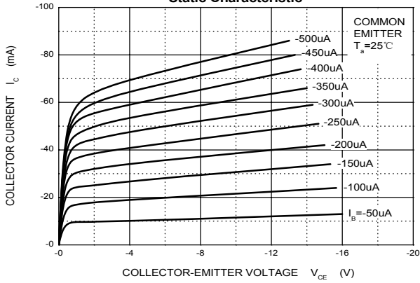
Static Characteristic
